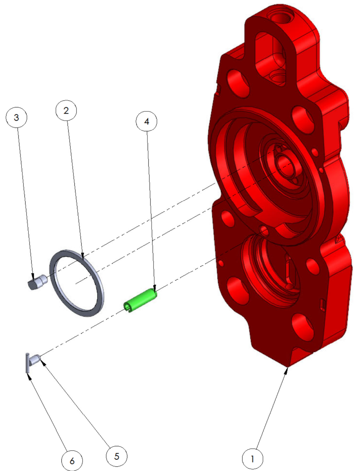
PUMP COVER CPL P#:180.02.02A
