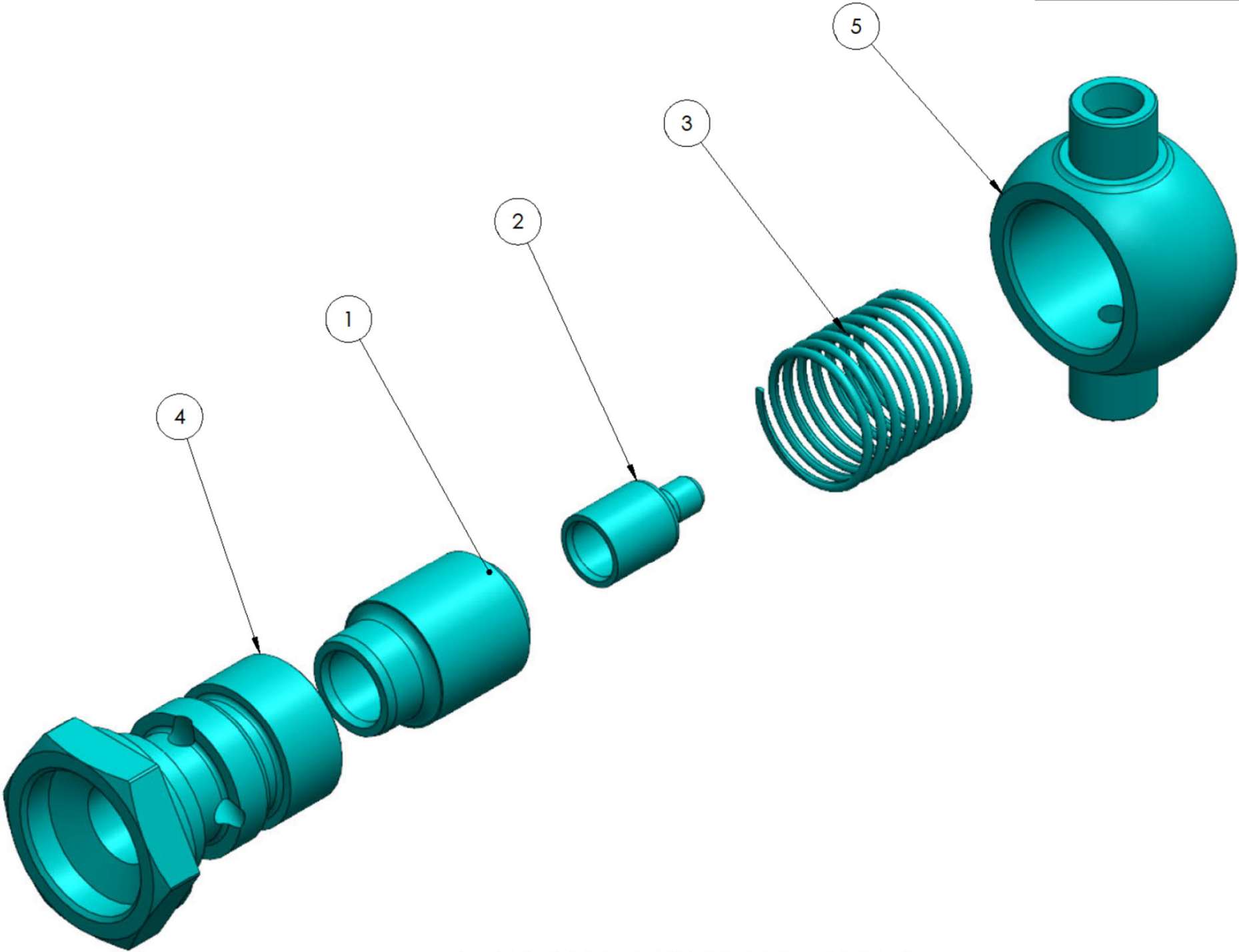
CHECK NON-RETURN VALVE CPL P#: 135.02.06
