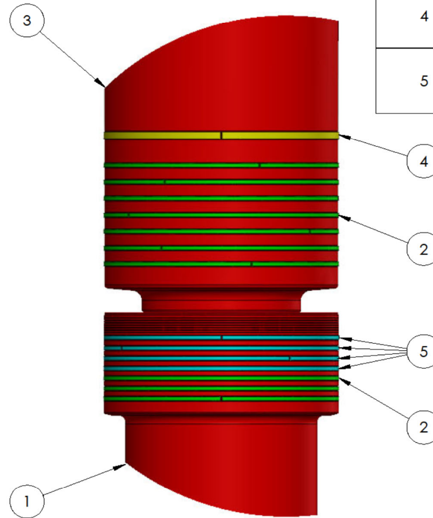
DETAIL A SCALE 1 : 15
