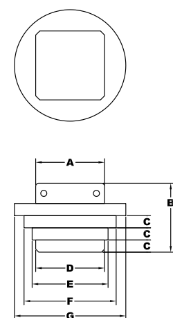
30" PIPE INSERT
